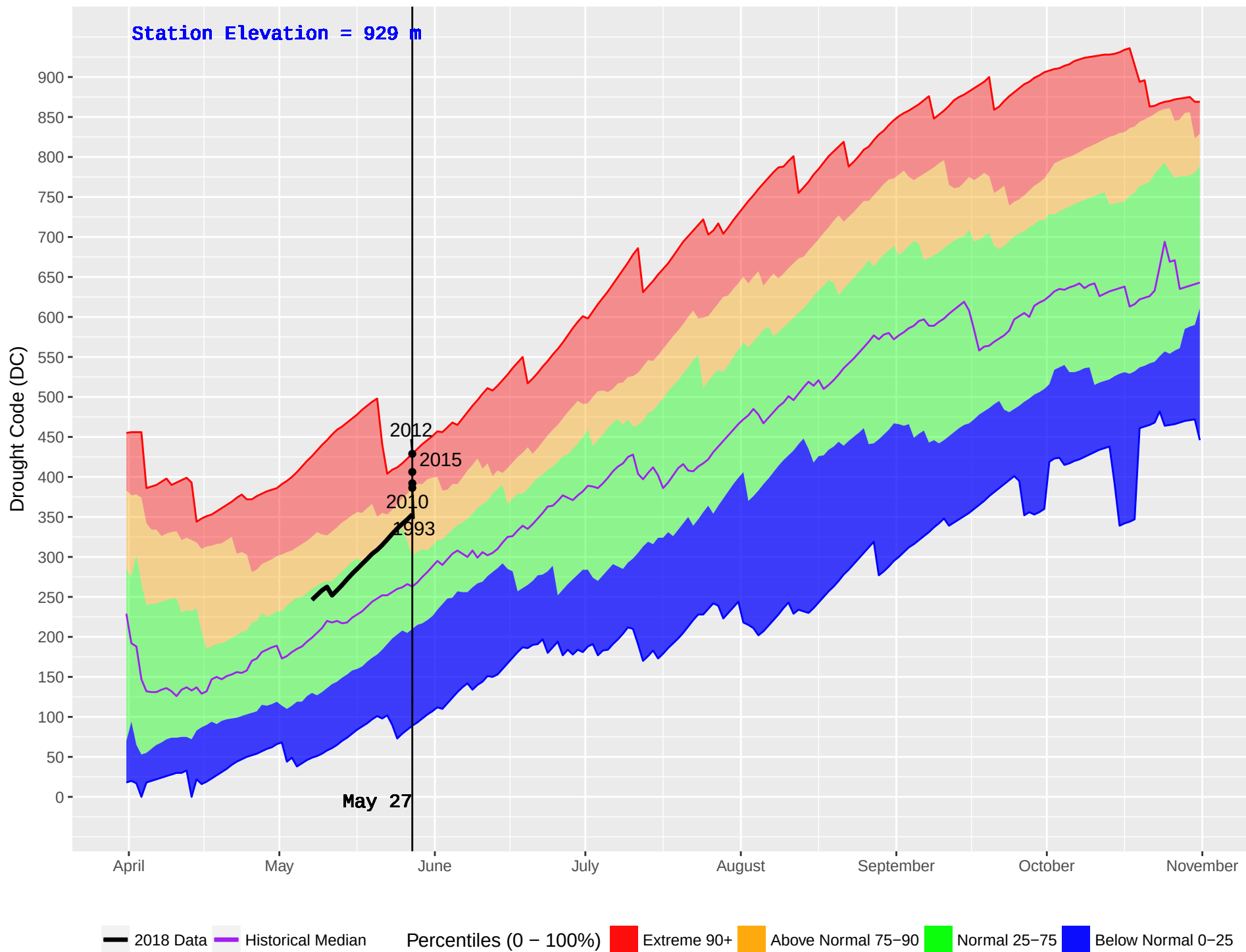
RISKE CREEK (210) : Historical (1980–2016) and Current (2018) Noon Drought Code (DC)
