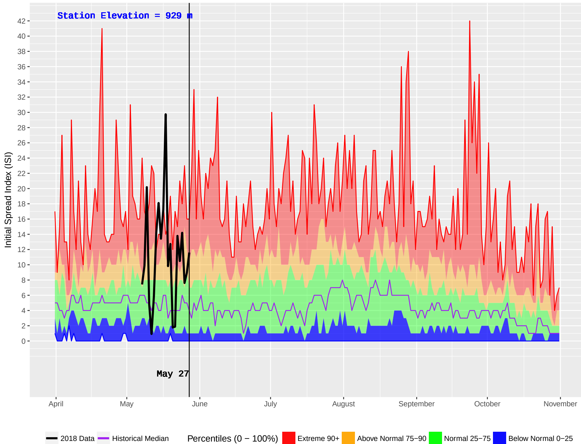
RISKE CREEK (210) : Historical (1980–2016) and Current (2018) Noon Initial Spread Index (ISI)
