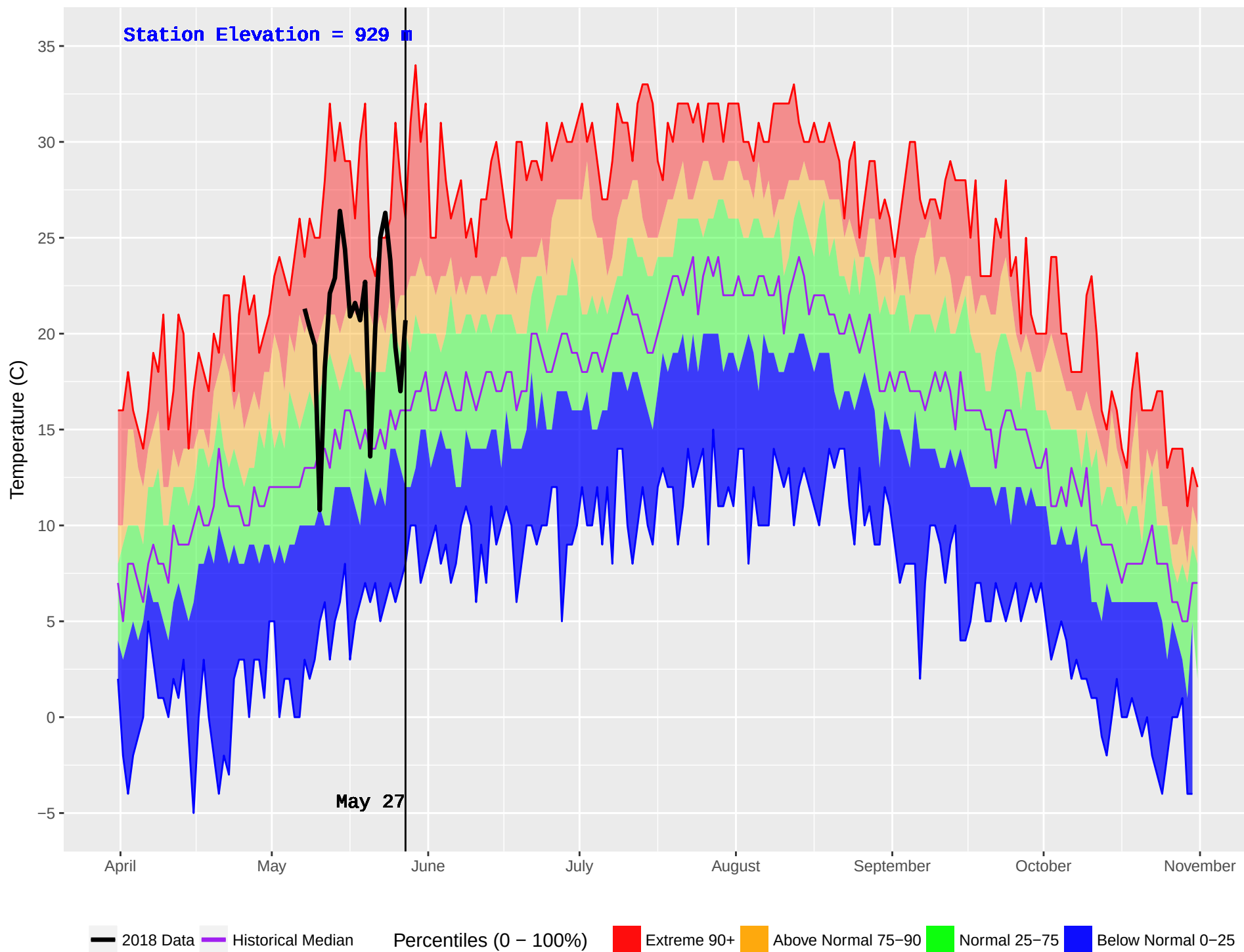
RISKE CREEK (210) : Historical (1980–2016) and Current (2018) Noon Temperature
