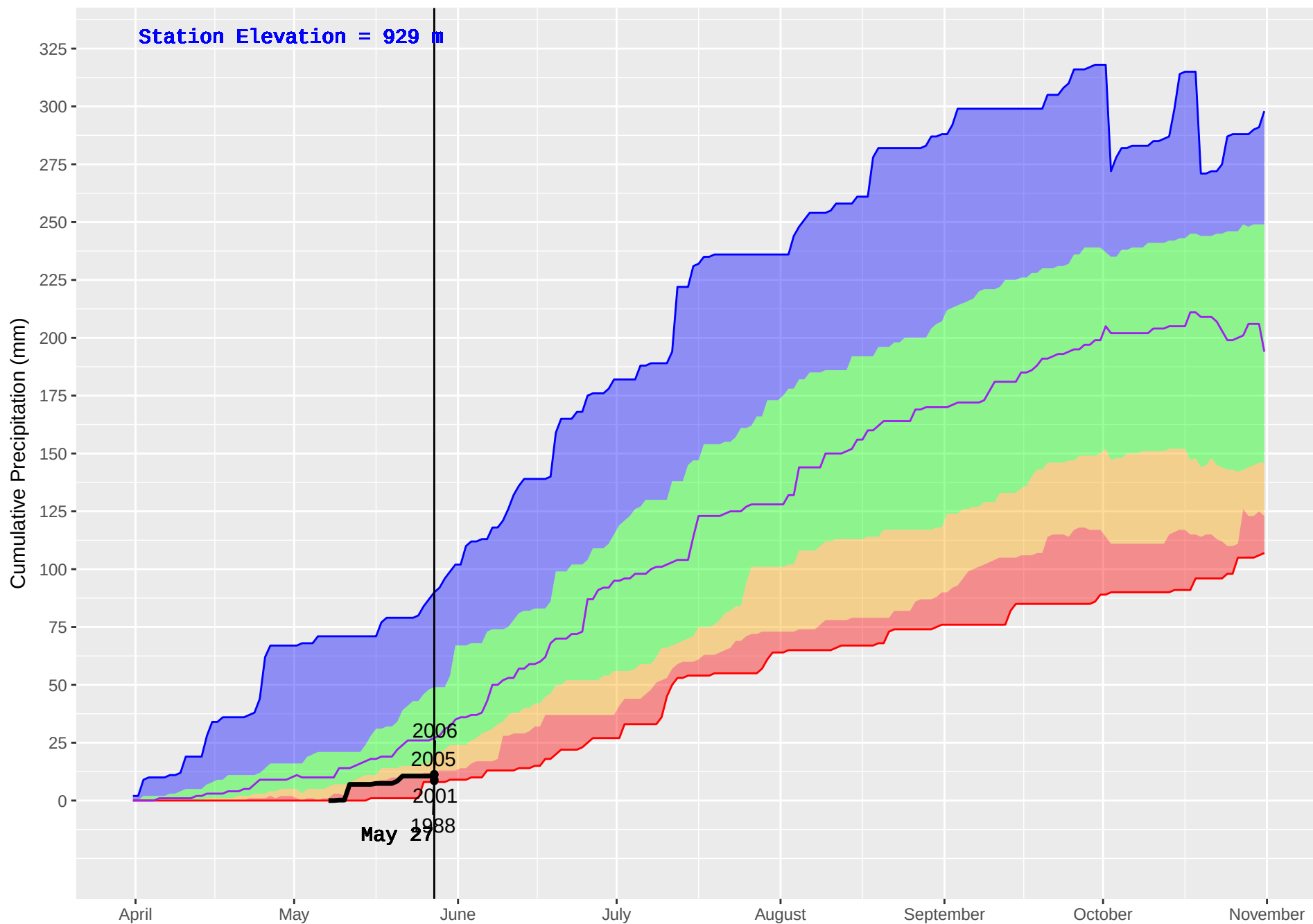
RISKE CREEK (210) : Historical (1980–2016) and Current (2018) Noon Cumulative Precipitation
