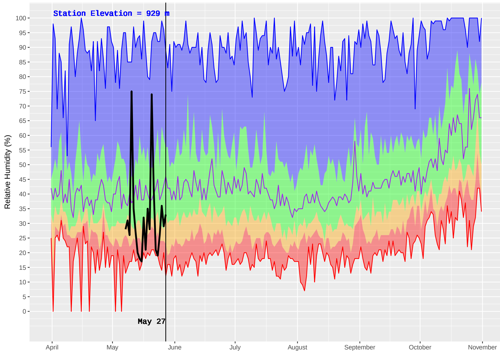
RISKE CREEK (210) : Historical (1980–2016) and Current (2018) Noon Relative Humidity
