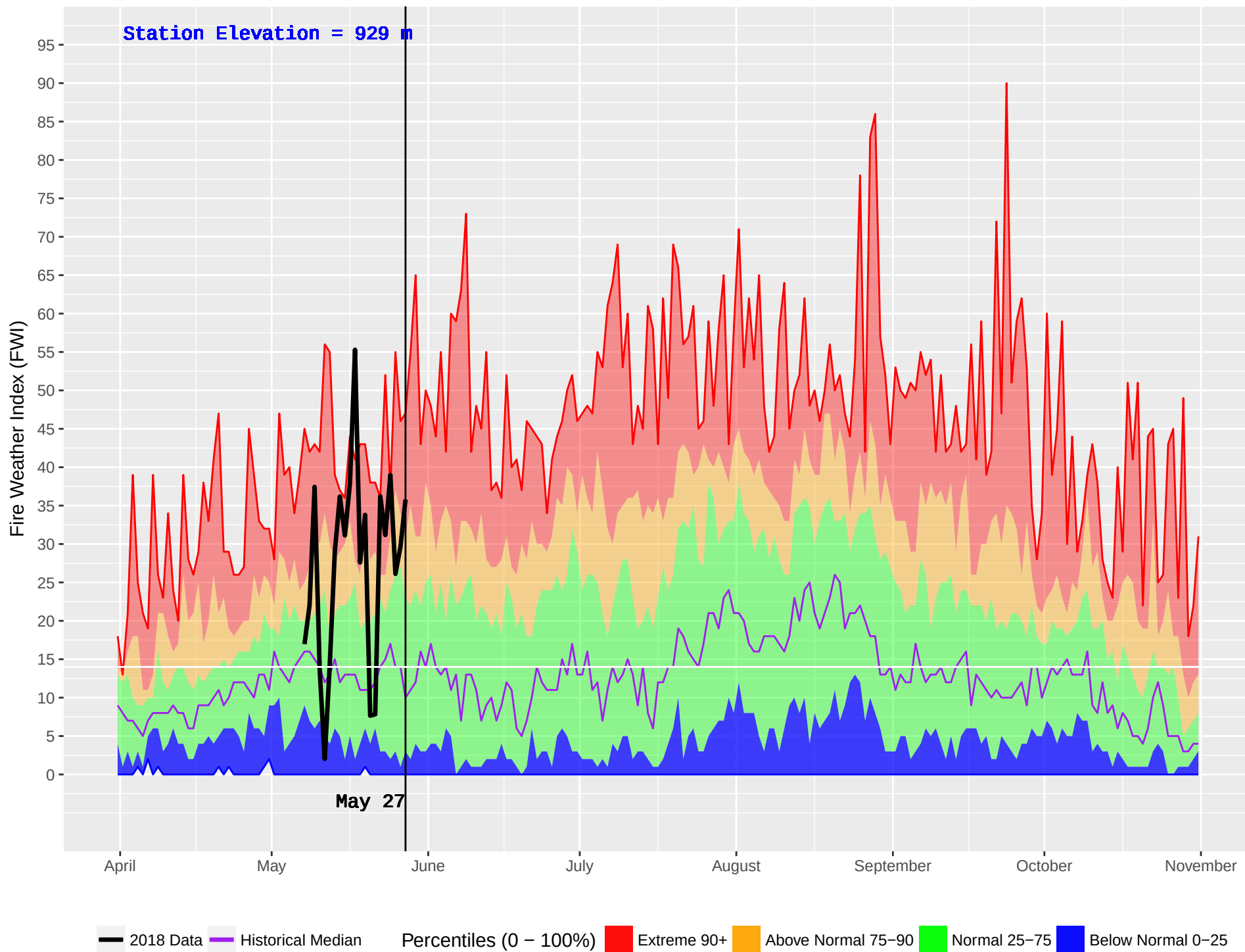
RISKE CREEK (210) : Historical (1980–2016) and Current (2018) Noon Fire Weather Index (FWI)
