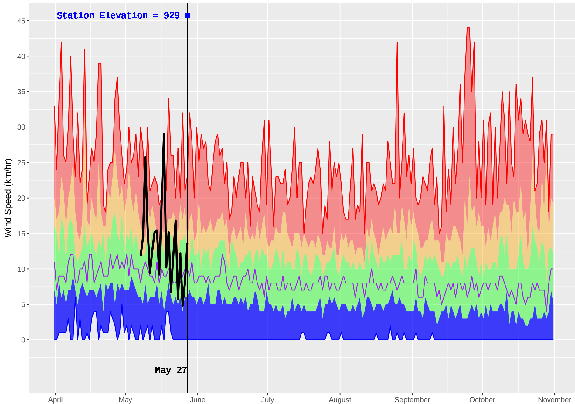
RISKE CREEK (210) : Historical (1980–2016) and Current (2018) Noon Wind Speed
