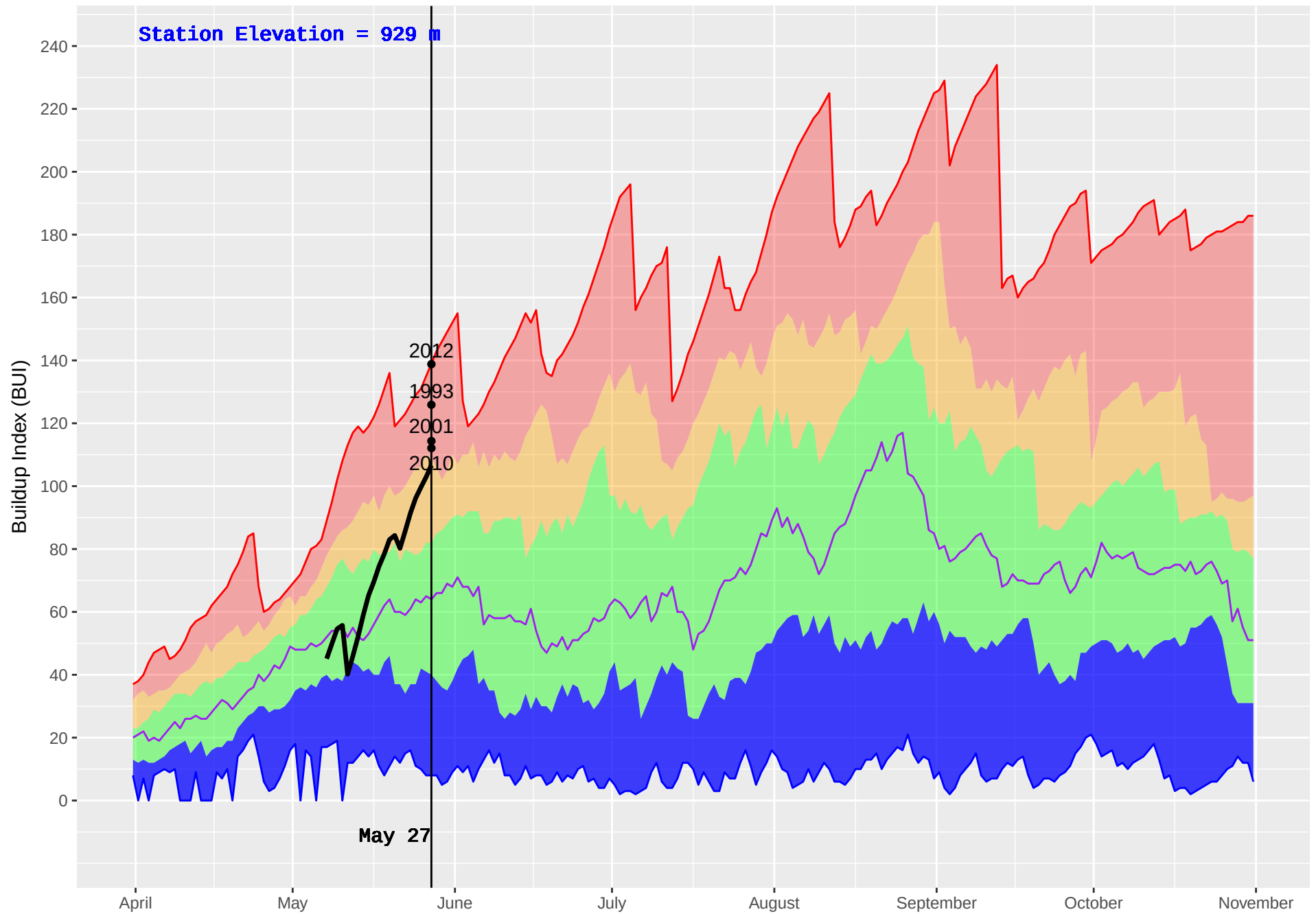
RISKE CREEK (210) : Historical (1980–2016) and Current (2018) Noon Buildup Index (BUI)
